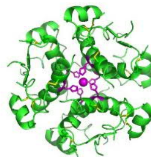
Insulinmolekyler
